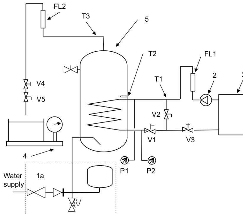
Figure F1.1 Apparatus example for unvented cylinder (EN12897) with internal coil type heat exchanger
