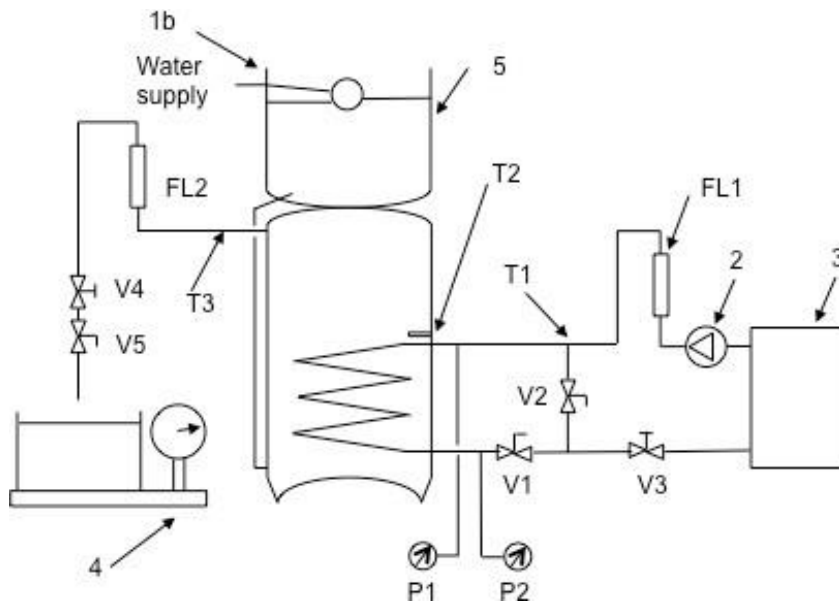
Figure F3 Apparatus example for copper combination unit (BS3198)
