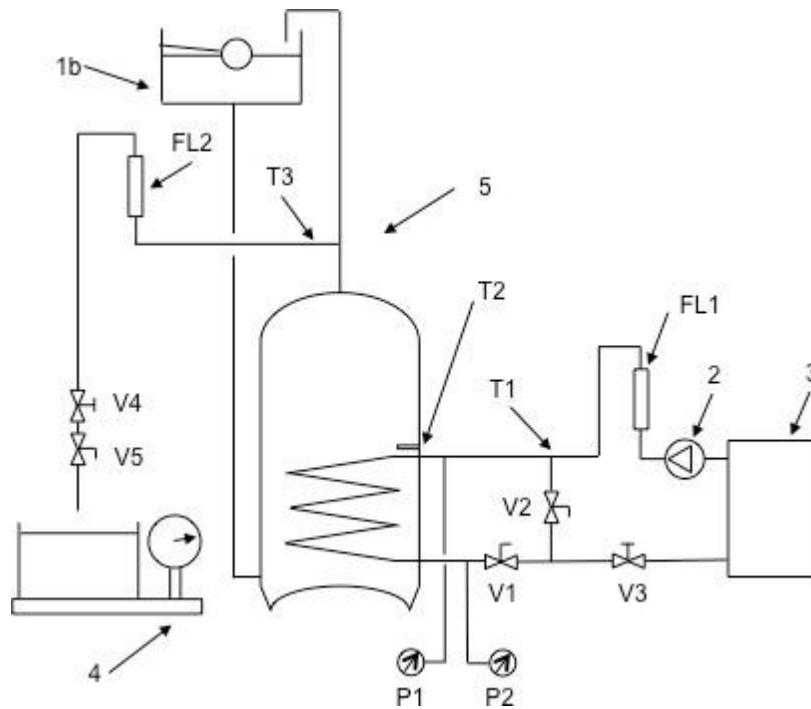
Figure F2 Apparatus example for copper or stainless steel vented cylinder (BS1566 or HWA 001)
